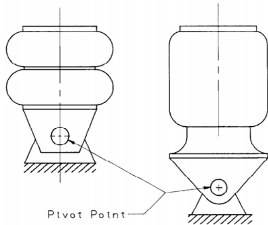
Fig. 5.9 Unstable mounting
