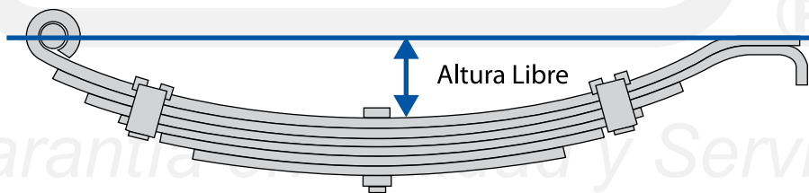
QTR-361m 2" X .323" X 14 1/4" X 16 3/8"
