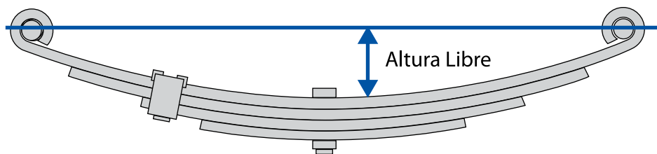
QTR-224 1 3/4" X .360" X 13 5/32" X 13 5/32" CAPACIDAD 2400 Lbs.
