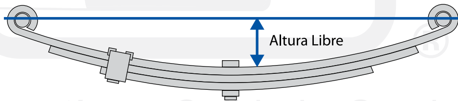
QTR-218 1 3/4" X .360" X 13 5/32" X 13 5/32" CAPACIDAD 1750 Lbs.
